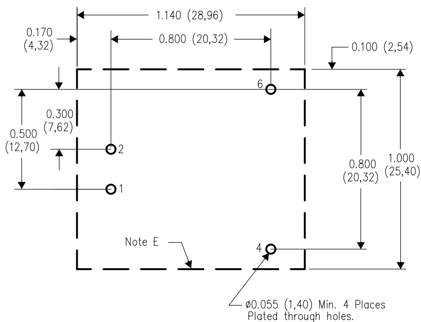
PC LAYOUT
